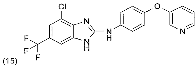
(4-Chloro-6-trifluoromethyl-1H-benzimidazol-2-yl)-[4-(pyridin-3-yloxy)-phenyl]-amin
